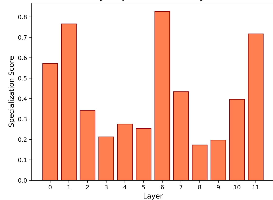
Layer Specialization Analysis
