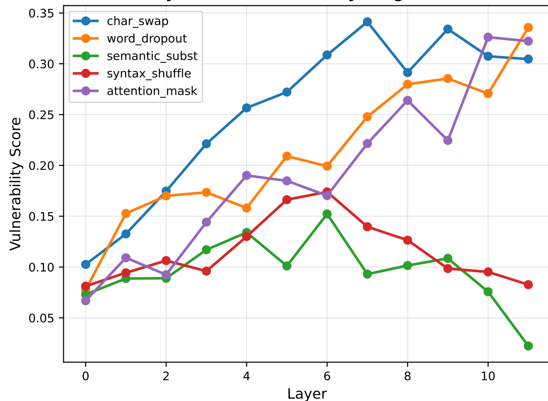
Layer-wise Vulnerability Progression
